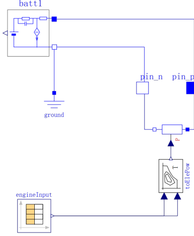
Figure 2: The energy consumption model
