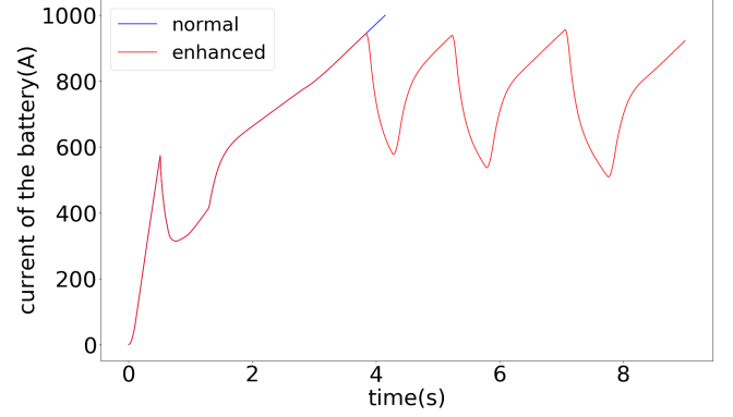
Figure 5: Runtime battery discharging of the vehicle
