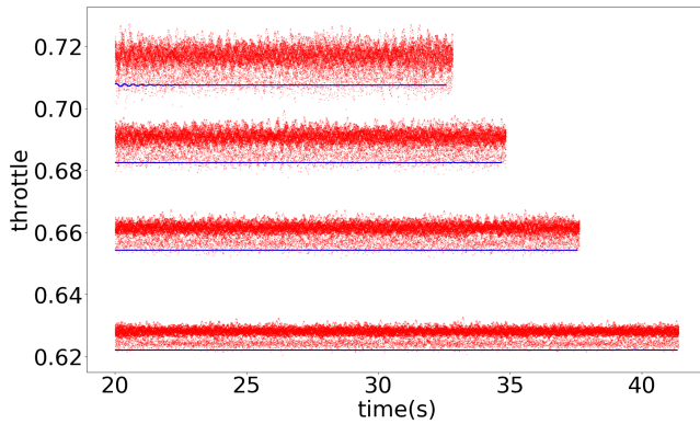
Figure 8: Throttle changes of the vehicle under the simulations of different speed limits
