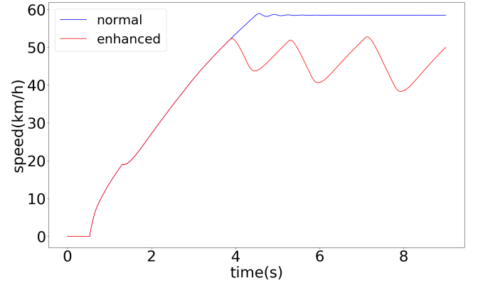
Figure 6: Runtime speed of the vehicle
